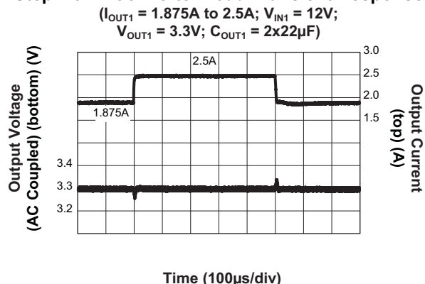
Step-Down Converter Load Transient Response
